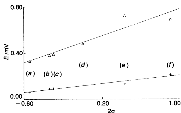
Fig. 13 Least-squares plots of E_{298}^{\alpha(1)} and E_{298}^{\alpha(2)} vs. 2\sigma for [\text{Co}(\text{OMeN}_3\text{C}_6\text{H}_4\text{X}-4)_2] chelates. X = OMe (a), Me (b), Et (c), H (d), Cl (e) and \text{CO}_2\text{Et} (f). \rho = 0.10 at E_{298}^{\alpha(1)} and 0.26 at E_{298}^{\alpha(2)} . The values of \sigma are taken from ref. 15
